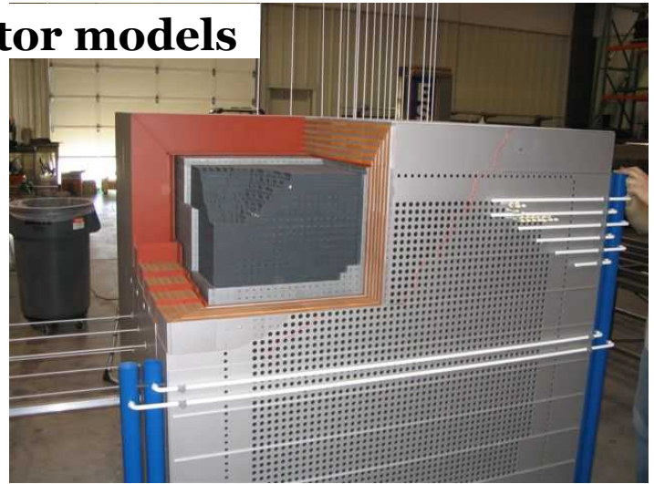
B Reactor model with pile cutaway
